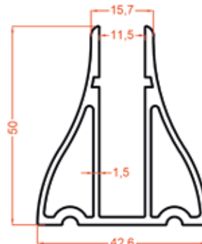
1374 1.030 Kg/m
