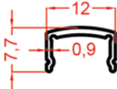
1706 0.412 Kg/m
