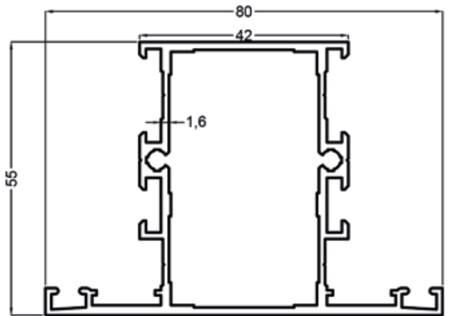
1859 1.260 Kg/m
