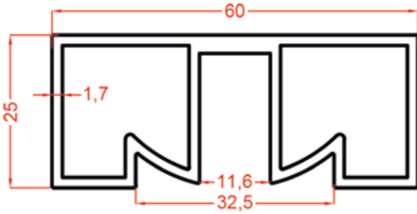
1401 1.005 Kg/m
