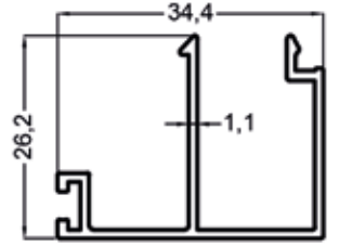
1860 0.309 Kg/m
