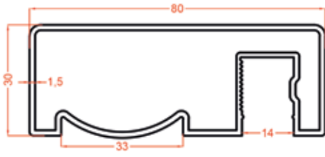
152-R1 1.076 Kg/m
