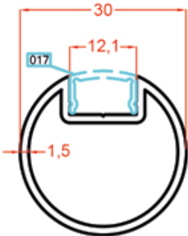
1706 0.412 Kg/m
