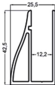
1763 0.615 Kg/m
