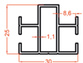
1593 0.385 Kg/m
